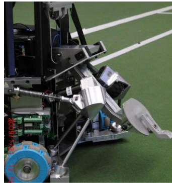
Fig. 14. Side view kicking mechanism, lob shot.
