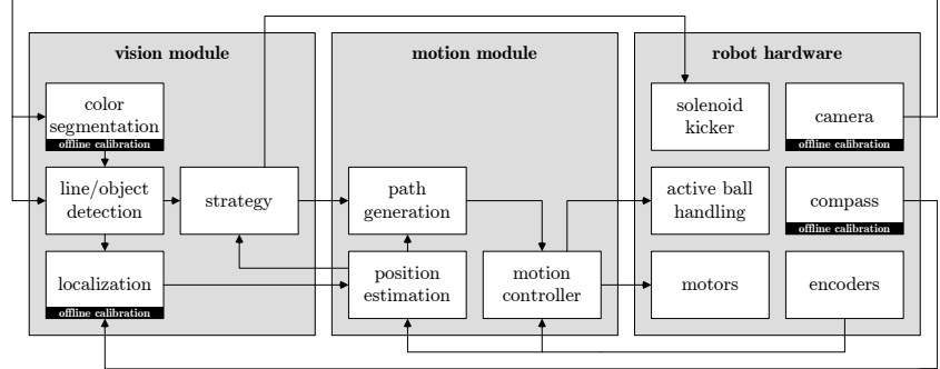
Fig. 2. A schematic scheme of the robot's hardware and software modules and their interconnections. Components that are field dependent and have to be calibrated offline are marked black.
