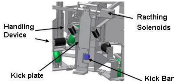
Fig. 3. Kick Device
