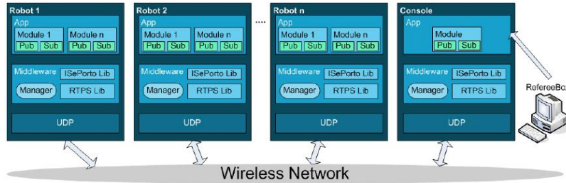
Fig. 1. Example of a typical RTPS communication system focusing the RoboCup's MSL
