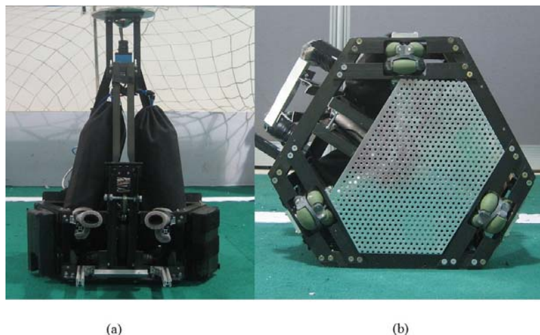
Fig.2 Our omni-directional soccer robot
