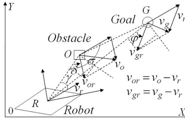
Fig. 7. Effect on APF caused by relative movement
