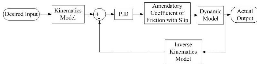
Fig. 4. Robot control structure
