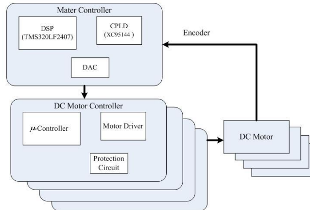
Fig. 5. Control system for the robot
