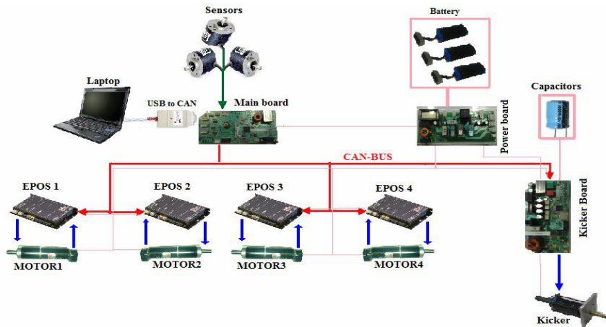
Fig . 2. Electrical and Control architecture
