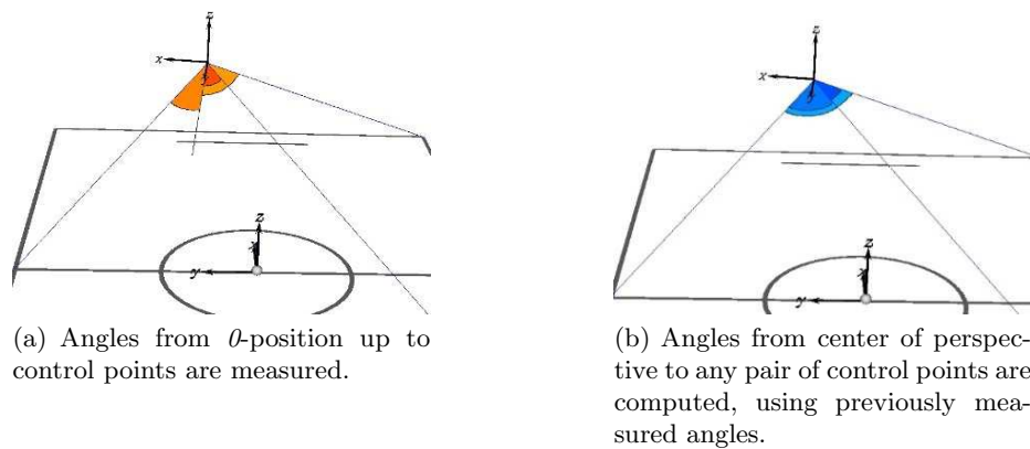
Fig. 2. Compute angles for Bolles and Fischler's method.
