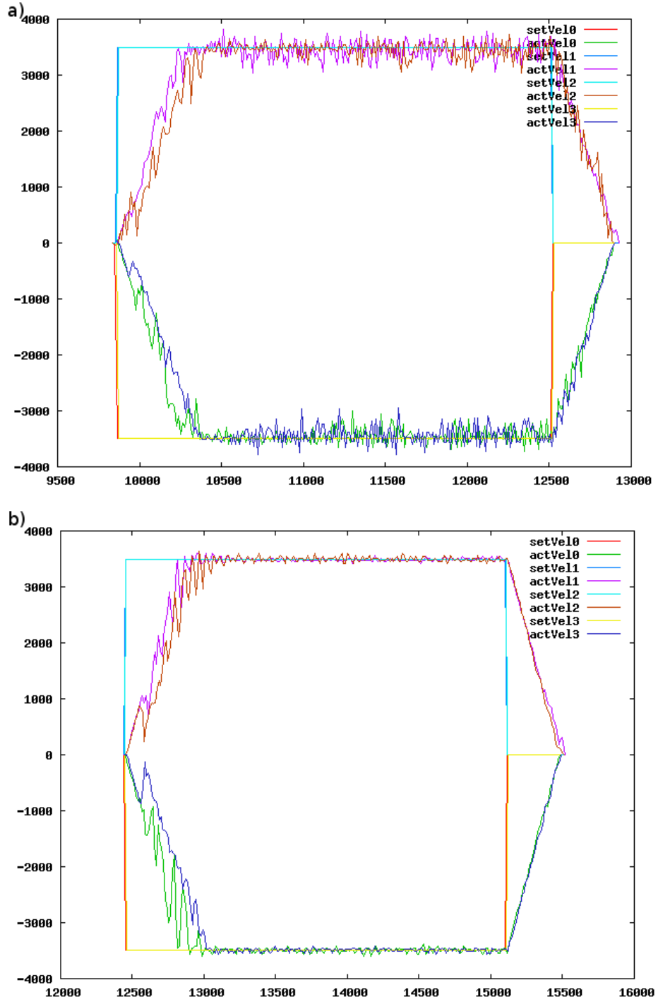
Fig.4. The diagramm shows the difference between the angular velocity set to the motors and the real values (measured by encoders [Max08]). a) poor PID-Parameters (delta between set and real values is high) b) optimal PID-Parameters (delta between set and real values is low)
