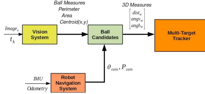
Fig. 2. Ball Estimation Architecture
