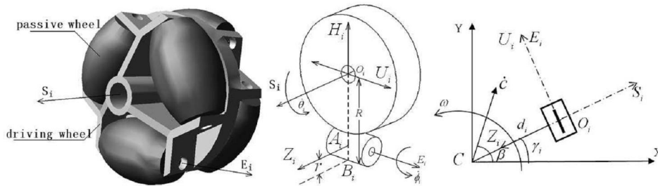
Fig. 4. Omni-directional wheel
