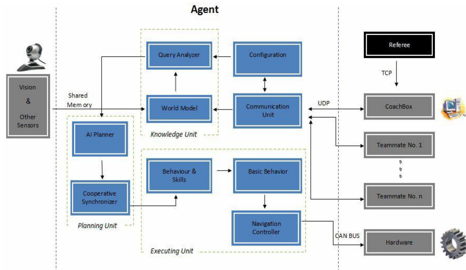
Fig. 4. High Level controller block diagram
