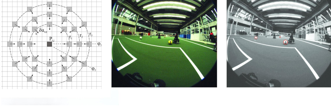
Fig. 6. Left: Principle of the ball detection algorithm. For a number of points on a circle with radius r around the pixel the derivative in the direction of the center point is calculated. The sum of these derivatives for radius r gives the confidence measure of a circle with a radius r being present at this pixel. Center: Example image from the front camera. Right: Image of the front camera with ball detection (Note that the blue ball is not detected due to the shape after the gradient operation).
