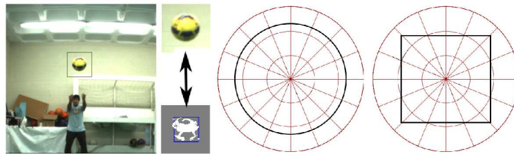
Fig. 3. Example of a ball detected using the front vision system and a graphical representation of the polar histograms used to validate the circularity.
