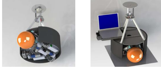
Fig. 2. The new platform of the CAMBADA robots.
