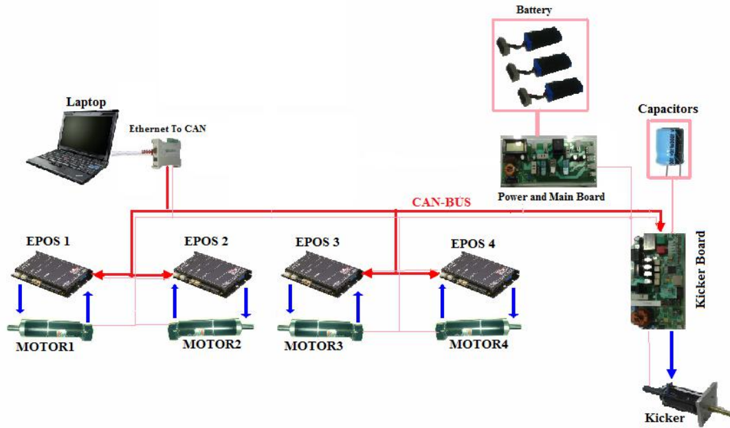
Fig . 3. Electrical and Control architecture
