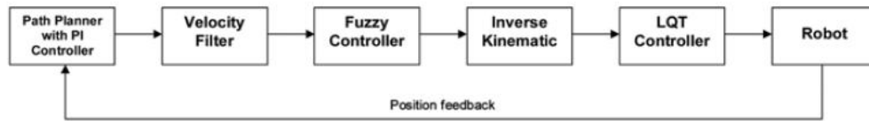
Fig. 2. MRL robot control diagram.
