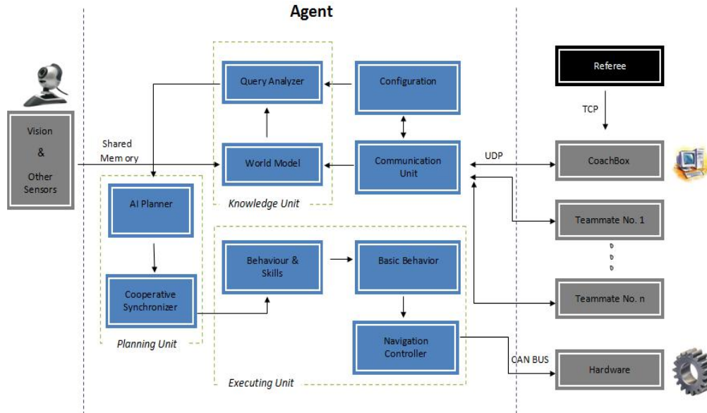
Fig. 5. High Level controller block diagram
