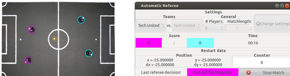
Fig. 3. Object-detection out of top-cam image (left), graphical user interface for autoref (right).
