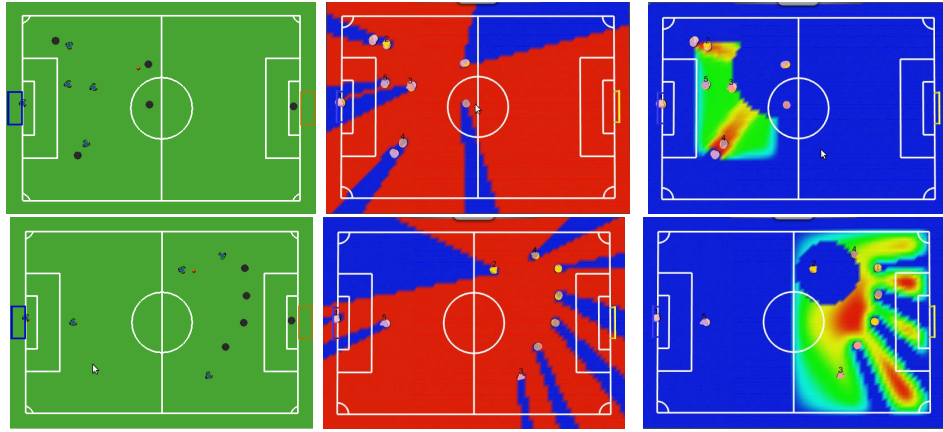
Fig. 4. Two game situations, the corresponding Field Of View based on the ball position and the height maps. The values are color code from blue to red, where red represents a highest utility value and blue the lowest. In the first row is a defending situation and in the second row an attacking situation.
