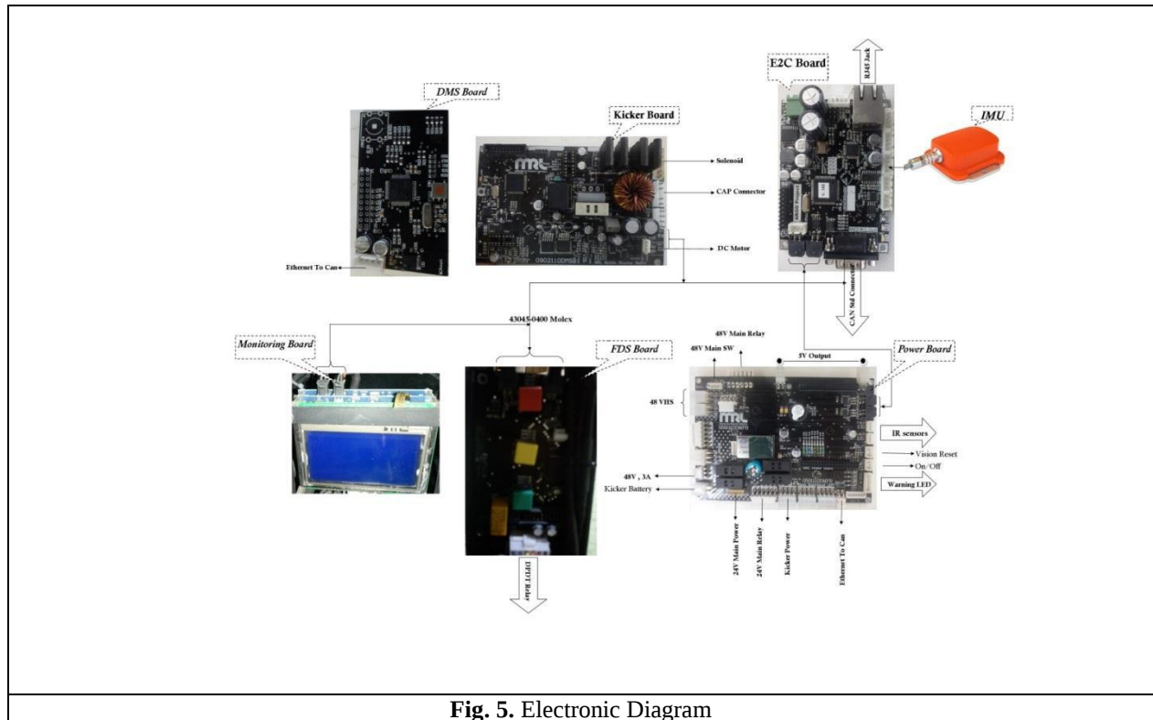
Fig. 5. Electronic Diagram
