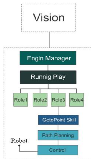
Fig. 7. Software architecture
