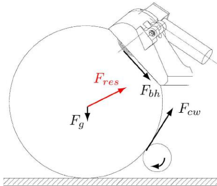
Fig. 5. Ball clamping forces.
