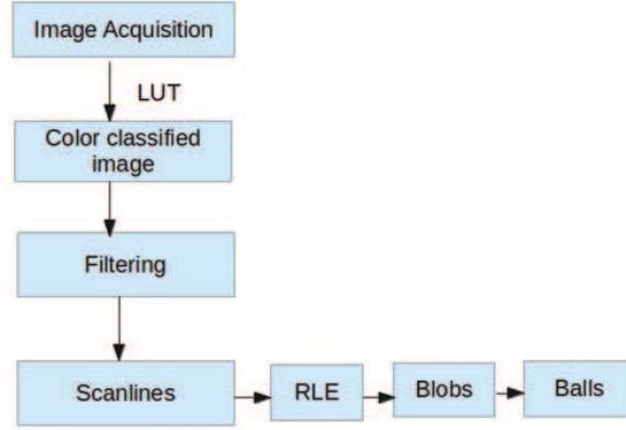
Fig. 1. Vision sytem pipeline of CAMBADA goalkeeper.
