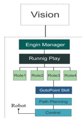
Fig. 7. Software architecture
