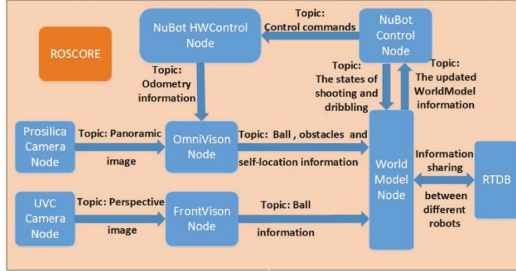
Fig. 6. The software framework based on ROS.
