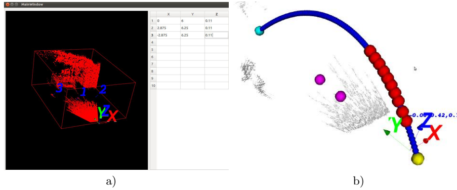
Fig. 5. On the left, the application for Kinect position calibration with 3 reference points on the Kinect cloud and the corresponding coordinates in robot coordinates system [8]. On the right, the calculated trajectory of the ball. The positions of the balls used for the computation are presented as large red spheres and the parabolic trajectory estimated is represented by the small blue spheres. The magenta spheres represent the projection on the ground of the detected balls.
