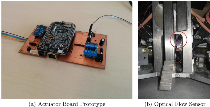
Fig. 5. Actuator Board and Optical Flow Sensor
