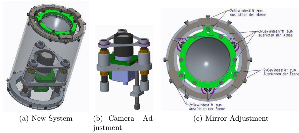
Fig. 4. The new Omni-Visio Concept
