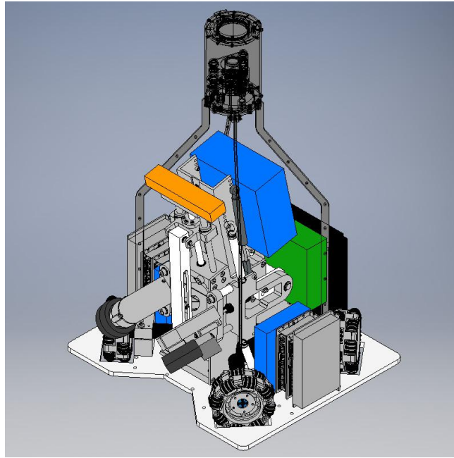
Fig. 2. Overview of the new Kicker and Ball-Handling Concept
