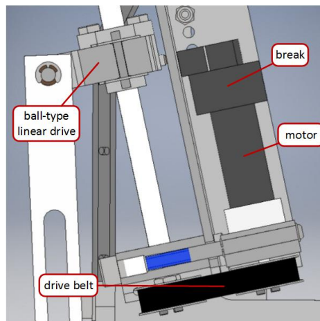
(a) Kicker Concept
