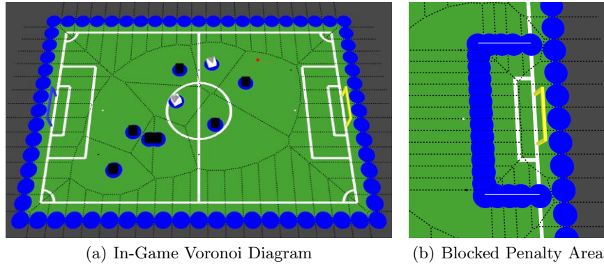
Fig. 1. Voronoi-Based Path Planning
