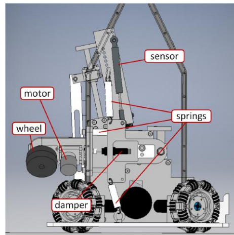
(b) Ball Handling Concept
