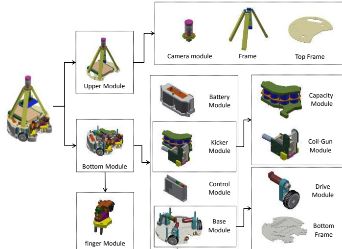
Figure 1. “Musashi” robot hardware configuration and modular architecture
