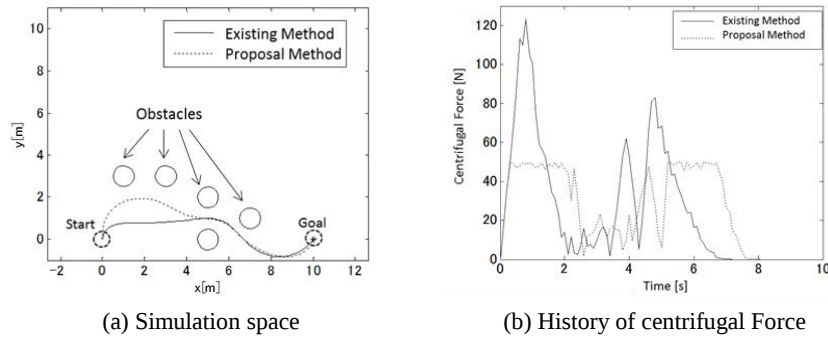
Figure 7. Simulation result
