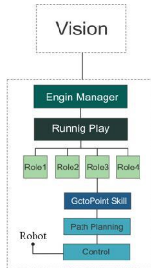
Fig. 7. Software architecture
