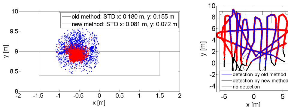
(a) Obstacle detection variation while the robot is moving across the field. (b) Obstacle detection range comparison while the robot is moving across the field.
