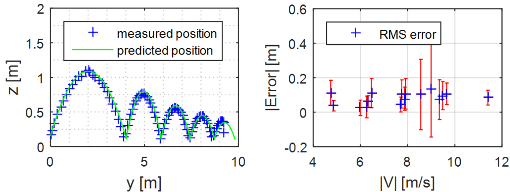
(a) Example of a comparison between a measured 2D ball trajectory and its predicted trajectory. (b) The RMS error between the measured and modelled paths for several measurements with different input velocities.
