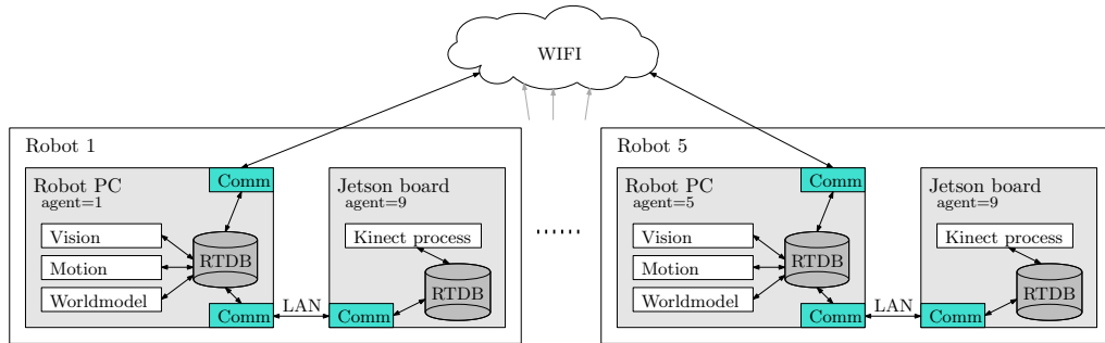
Fig. 3. Inter-process and inter-robot communication architecture using RTDB.
