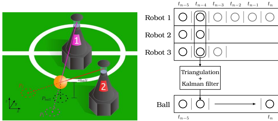
(a) Graphical representation of omnivision camera data triangulation. (b) A schematic representation of the triangulation algorithm.
