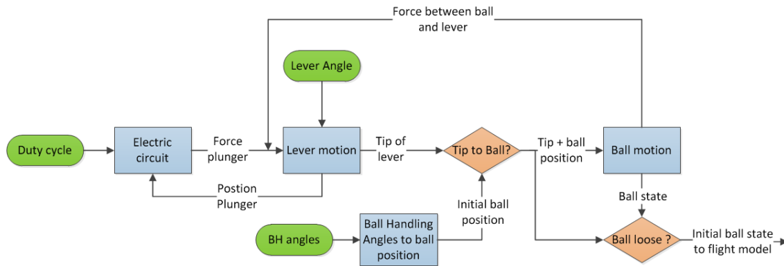
Fig. 6. Flowchart of the interaction between the robot and the ball.
