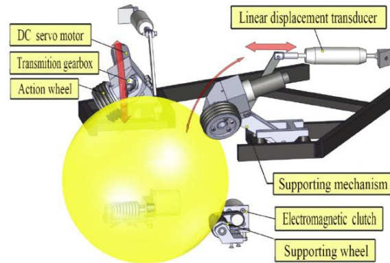
Fig. 3. Our active ball handling system.
