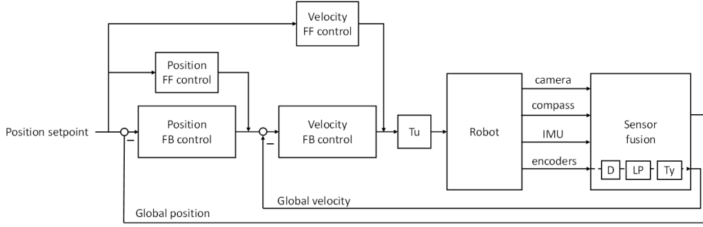
Fig. 5: Cascade control structure.
