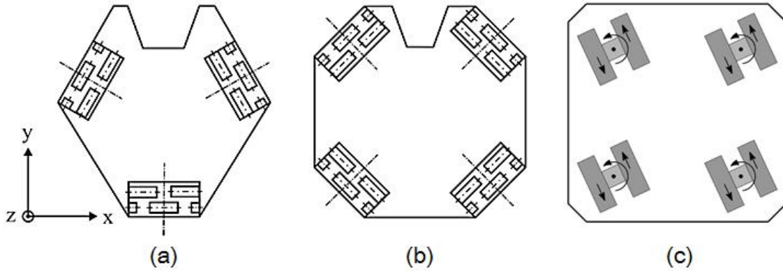
Fig. 2: Visualization of the different types of platforms: three-wheeled (a) and four-wheeled (b) with omni-wheels as discussed in [1] and the newly developed eight-wheeled platform (c) with four suspended wheel-combi's, able to rotate around a center hinge.
