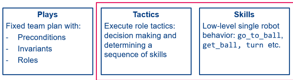
Fig. 3: A Play is a predefined team plan. Tactics and Skills together define the behavior of a single robot.
