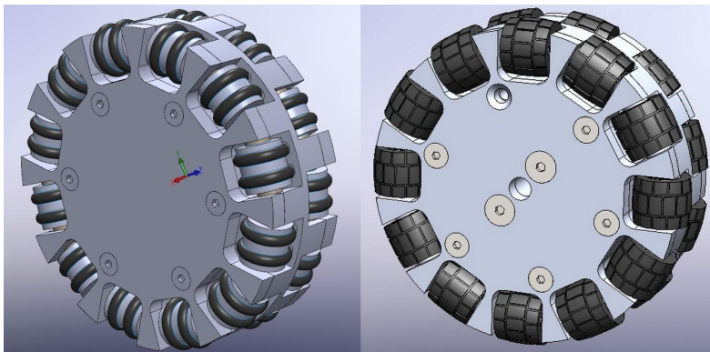
Fig. 1: New robot wheels.
