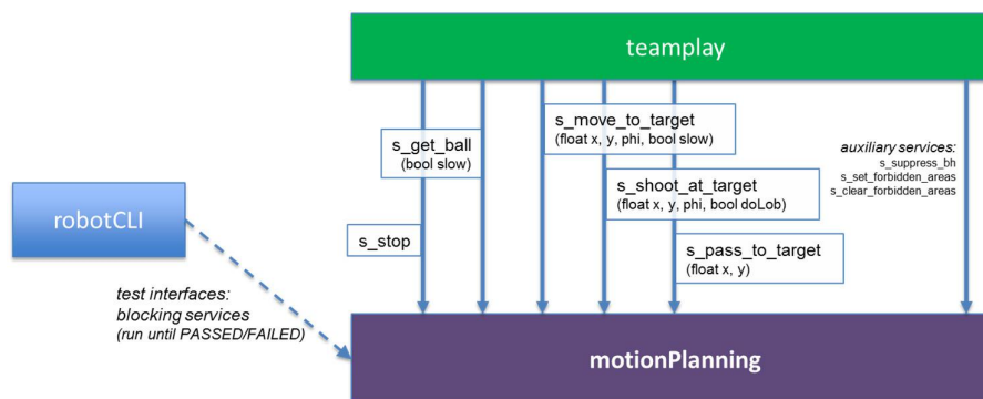
Figure 3 teamplay - motion planning interface
