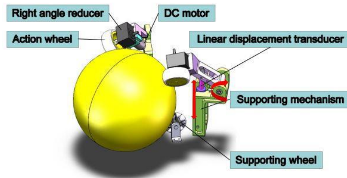
Fig. 2. Our active ball handling system.
