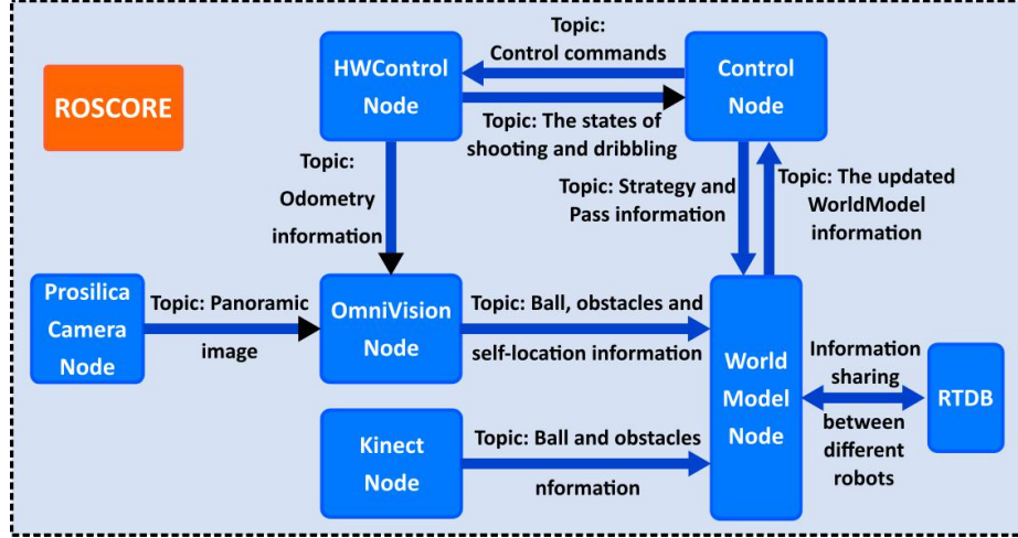
Fig. 2. The software framework based on ROS.
