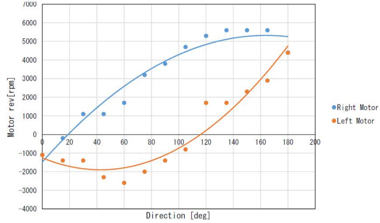
Fig. 5. Relationship of motor rev of ball handling module and direction that robot is moving
