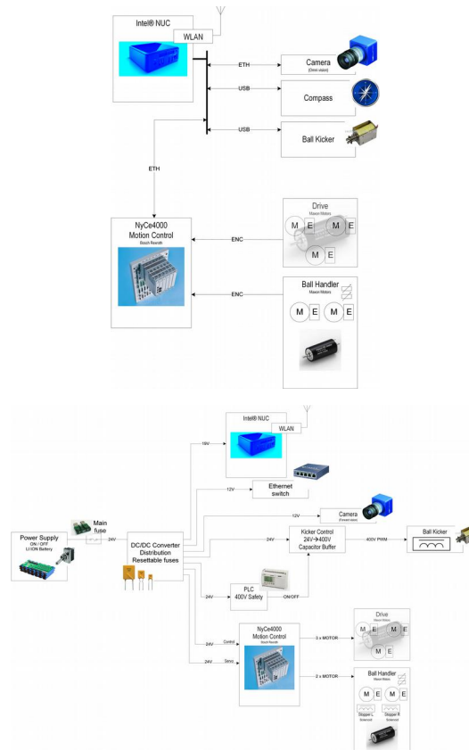
Fig1. Robot architecture with main building blocks, data and power flows
