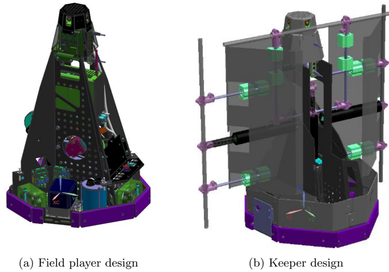
Fig. 5: Mechanical robot architecture
