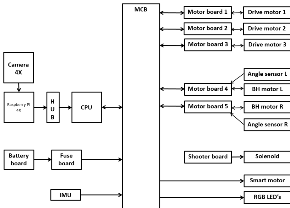
Figure 5: Communication flow
