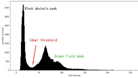
Fig. 4: Intensity histogram of the image
