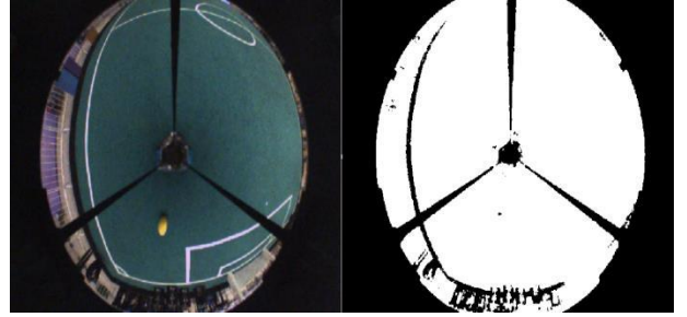
Fig. 5: Black obstacle extraction results
