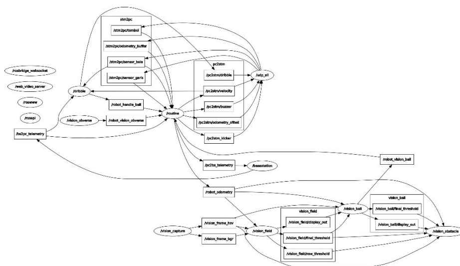
Fig. 5. Program Architecture
