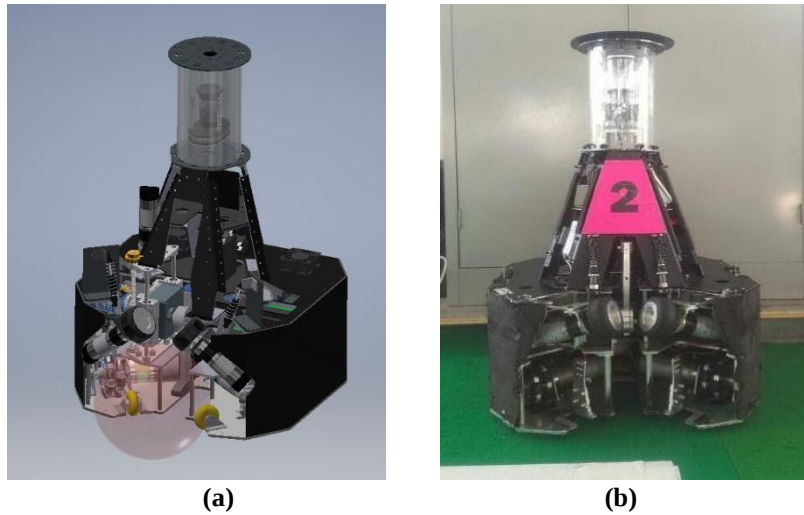
Fig. 1. (a) Second-Gen. Design of the Robots (b) Robot Photograph
