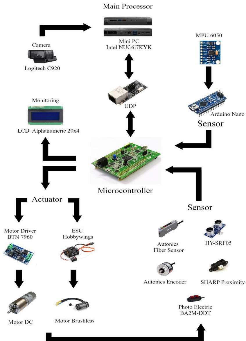
Fig. 4. Electrical System of the Robot
