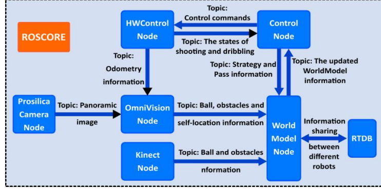
Fig. 4. The software framework based on ROS.
