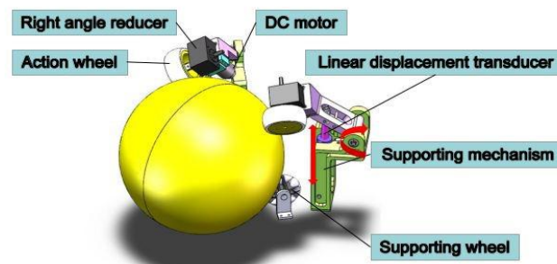
Fig. 2. Our active ball handling system.
