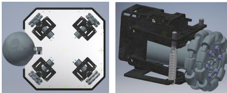
Fig. 2. New wheel configuration (left) and detail of wheel unit with suspension (right).
