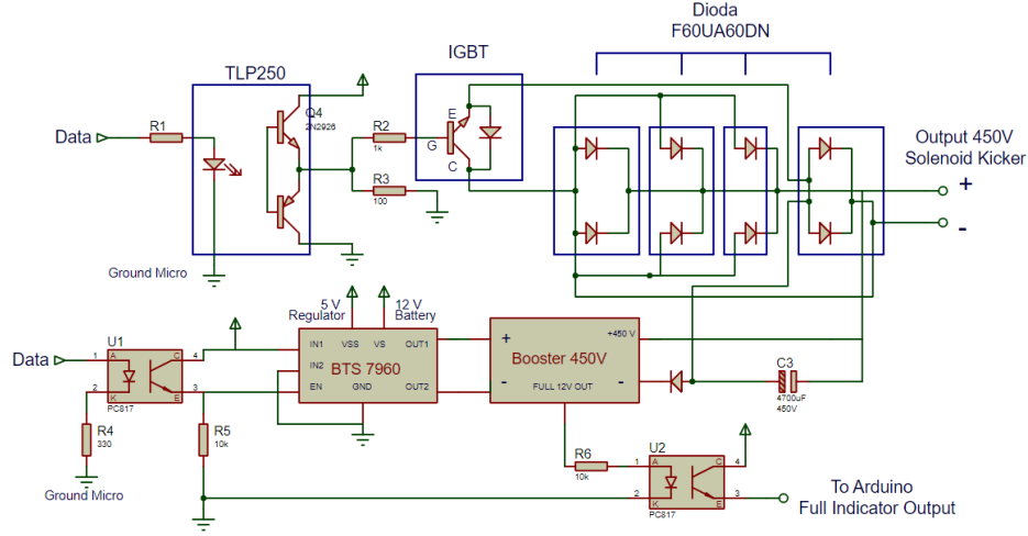
Figure 2. Schematic Driver Solenoid Kicker
