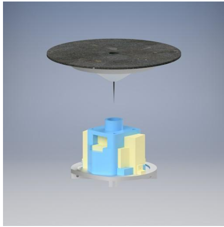
Fig. 3. Mechanical build of the top vision system.
