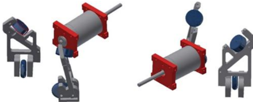
Fig. 4: Kicking and dribbling system design
