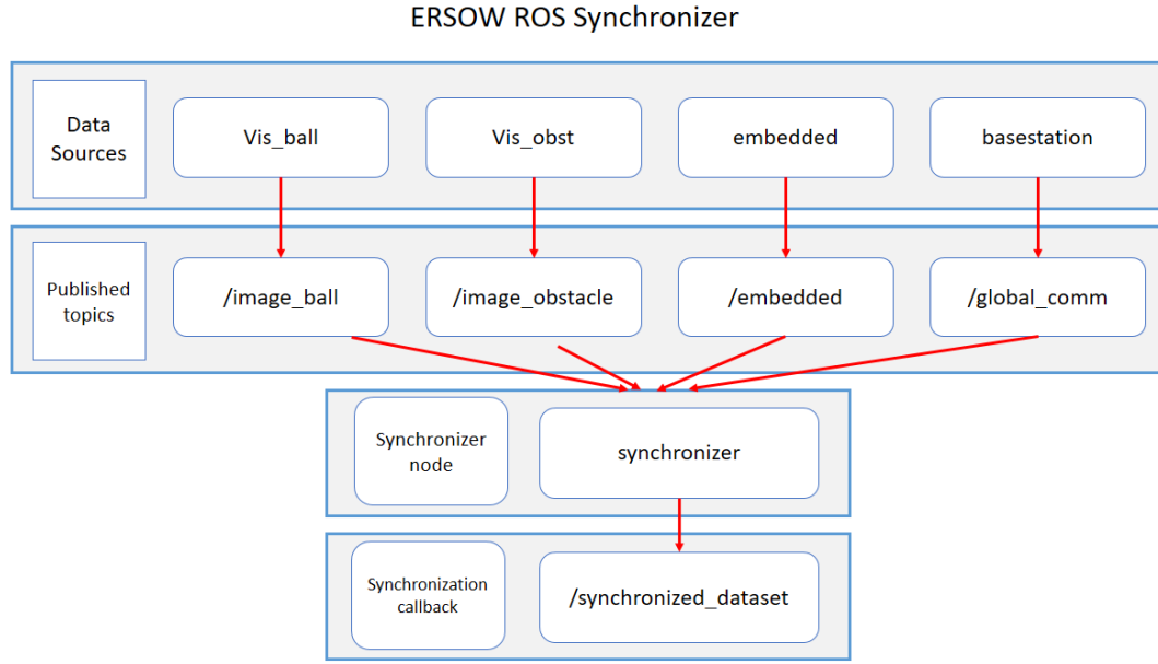
Fig. 7: Synchronization Design
