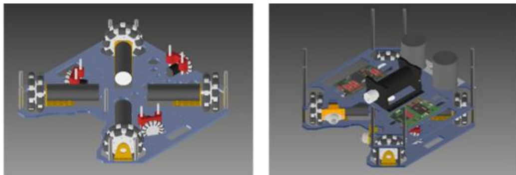
Fig. 2: Body-base robot
