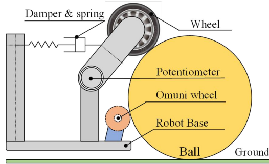
Fig. 2. Side view of Ball Handling Mechanism
