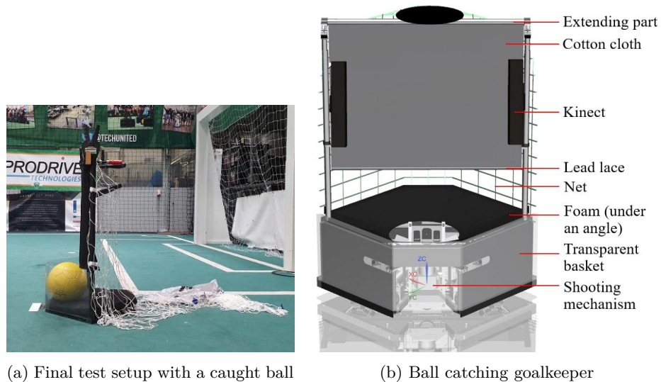
Fig. 3: Ball catching design
