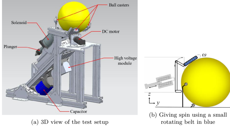
Fig. 1: Setups for shooting effect balls
