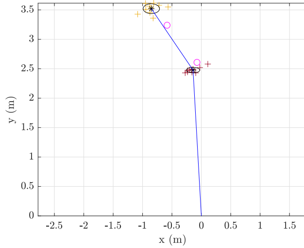
Fig. 2: Measurement of eight effect shots with the same settings. The predicted bounce locations are represented by \circ , the actual first and second bounce locations are indicated by respectively + and + , and the path of the ball is represented by (-) . The mean actual bounce locations are shown as * . The spin of the ball is 35.3 rad/s and the duty cycle is 22.2%.
