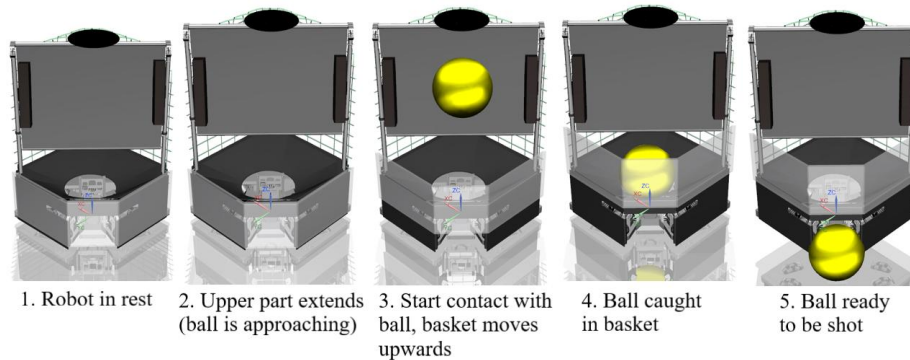
Fig. 4: Visualization of the working of the new designed robot in five stages
