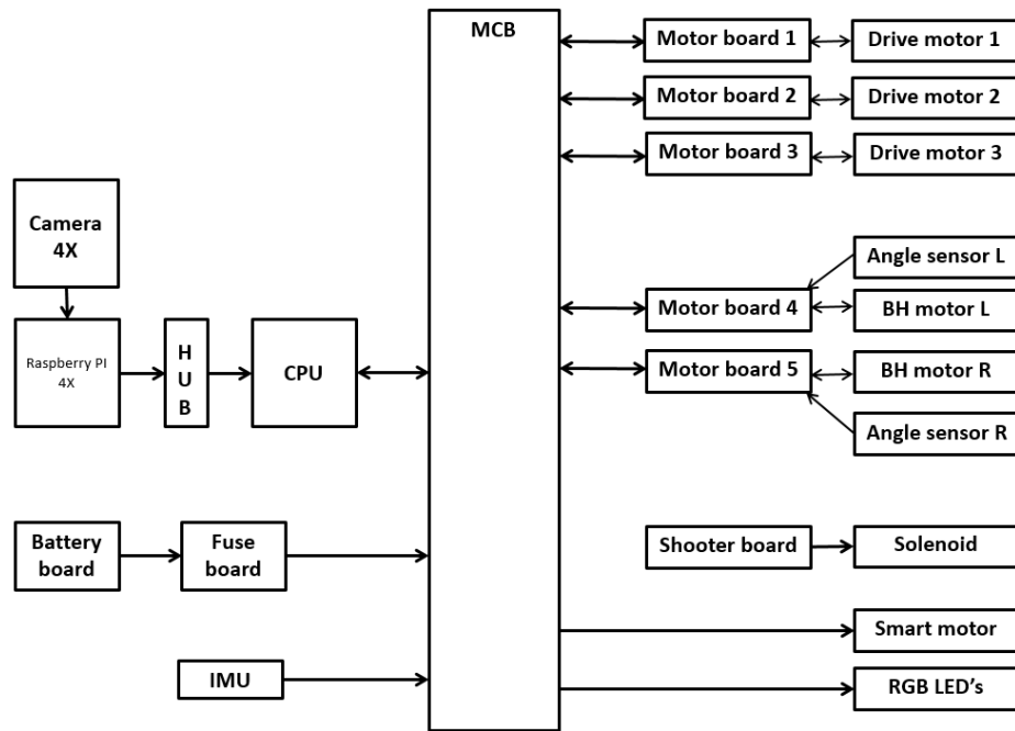
Figure 5: Communication flow
