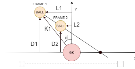
Fig. 4. Goalkeeper - Ball Trajectory Prediction
