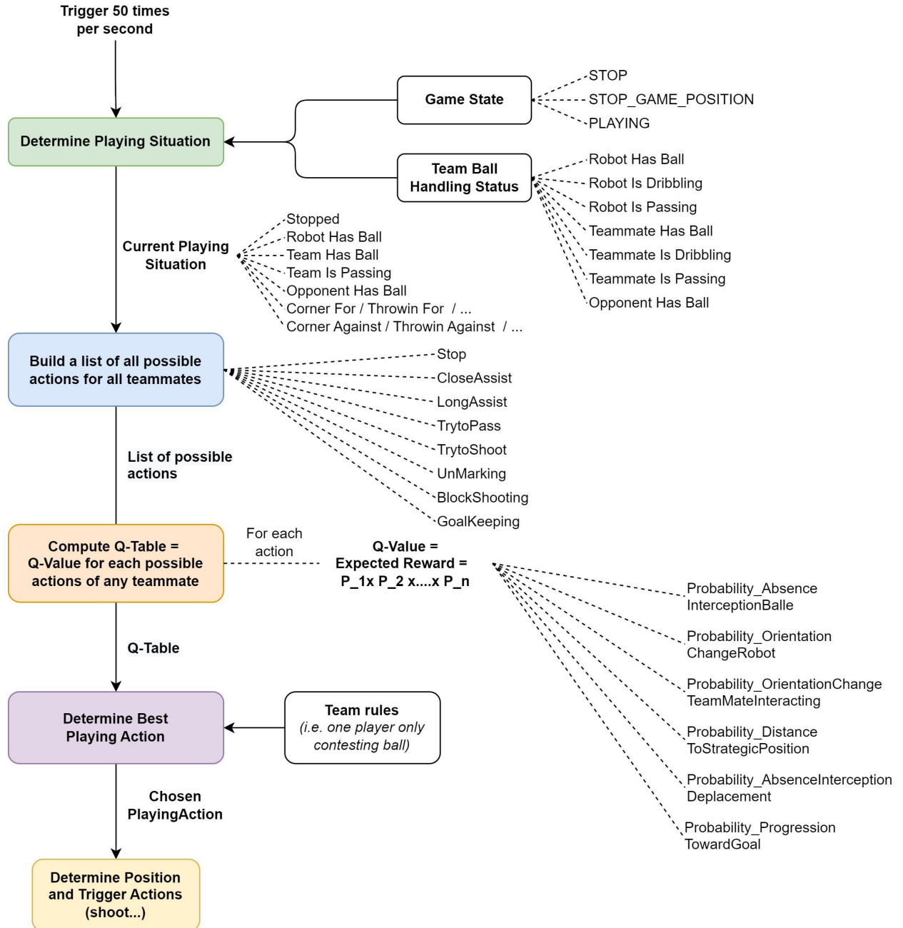
Fig. 7. Strategy algorithm of RCT team
