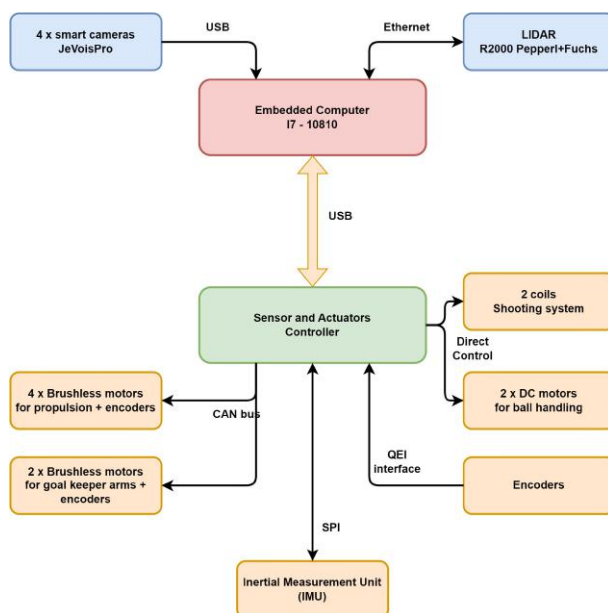
Fig. 2. RCT robots electronic bio-inspired architecture
