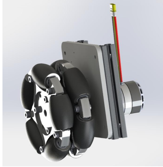
Fig. 5. RCT propulsion element
