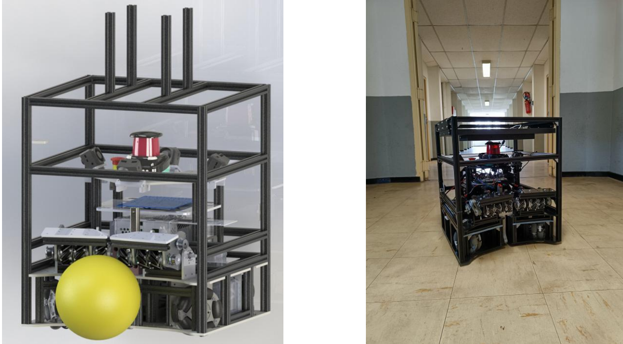
Fig. 1. Computer image of the 2022 robot of Robot Club Toulon Team, and picture of the robot.
