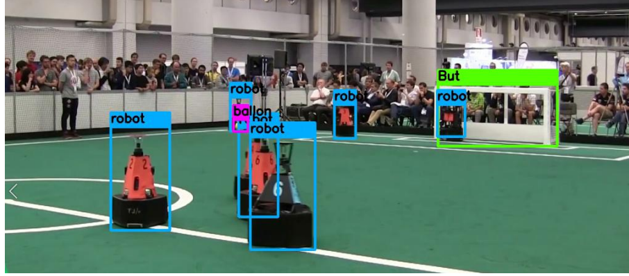
Fig. 6. Object detection result
