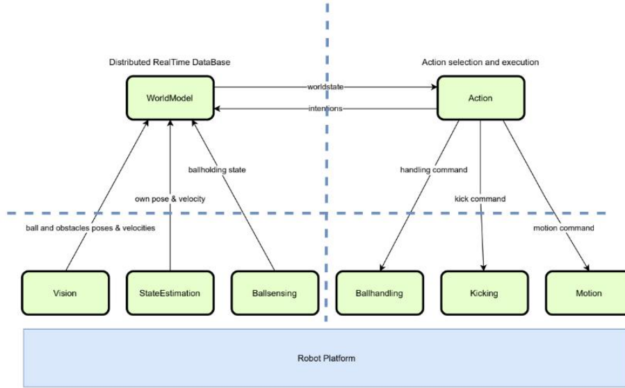
Fig. 3. Soccer Robot Architecture (Source: Eric Dortmans, Fontys)
