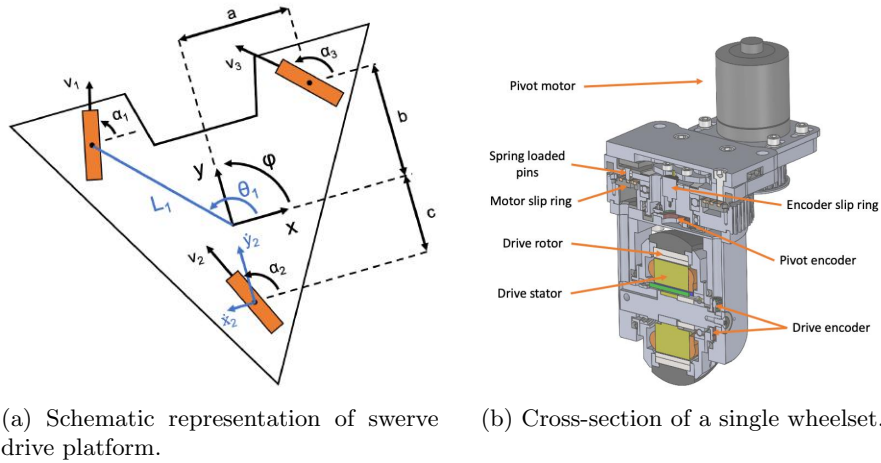
Fig. 2: Design and realisation of a robust, outdoor motion platform.
