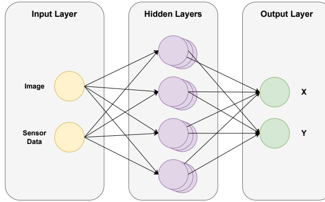
Fig. 9: Neural network architecture for robot self-localisation. Input data, including camera images and sensor readings, are processed through hidden layers to predict the (x, y) position of the robot within the environment.
