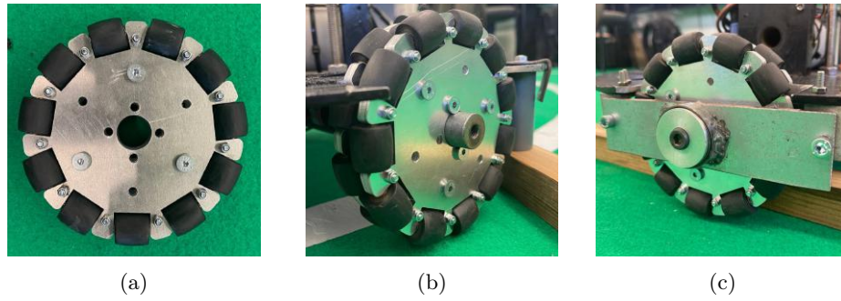
Fig. 1: Omni-Wheels: (a) One wheel assembled; (b) Wheel mounted on the robot; (c) Wheel with the outside bearing.
