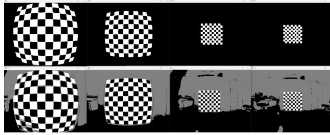
Fig. 7: Camera intrinsic parameter discovery process. Upper images: Simulated camera images. Lower images: Real-world images captured at different distances. The developed code facilitated accurate alignment between simulated and real-world perspectives.
