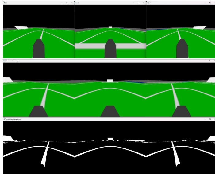
Fig. 8: Image processing pipeline. Top row: Three raw camera images captured without any filter or lens deformation. Middle row: Lens deformation applied to the images, followed by concatenation to form a panoramic view. Bottom row: Binary filter applied to the concatenated image to enhance feature detection and segmentation.
