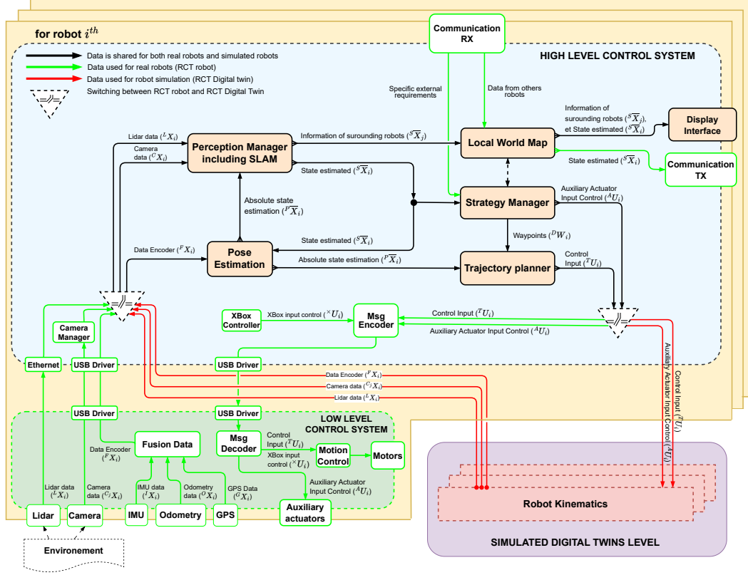
Fig. 3. RCT robots software architecture
