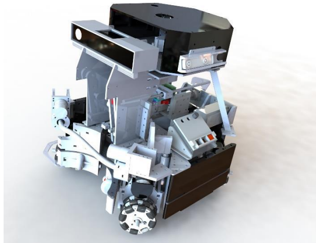
Fig. 1. Robot construction
